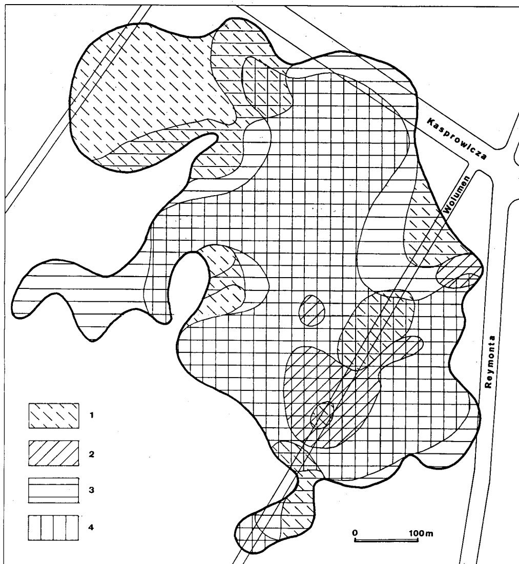
Fig. 4. Sketch showing the extent of various lithological types of the organic sediments of the Eemian buried lake in Wawrzyszew: 1 - lacustrine chalk, 2 - peats, 3 - gytja, 4 - bituminous shales
