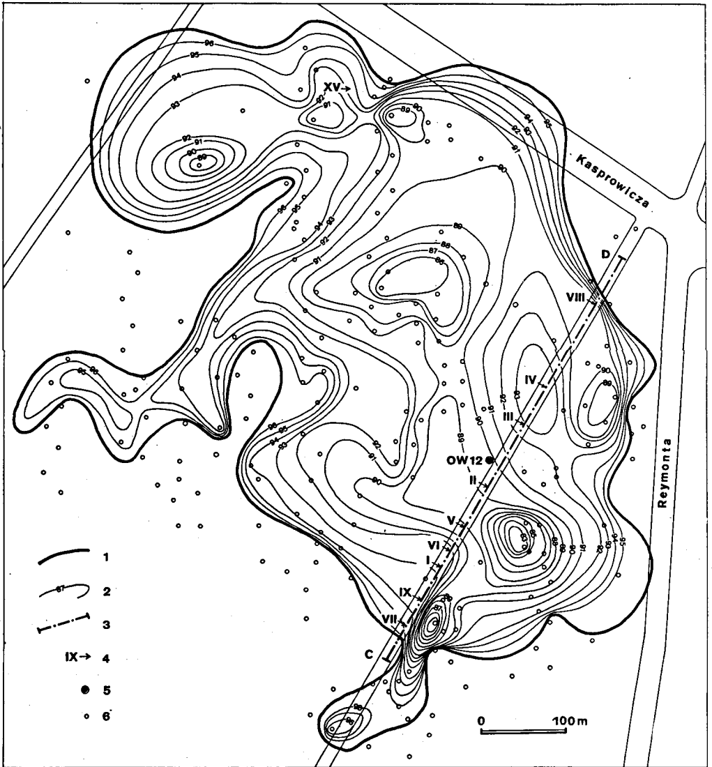
Fig. 3. Sketch showing the bottom relief of the organic sediments of the buried lake in Wawrzyszew (Eemian Interglacial): 1 – extent of the organic lacustrine sediments, 2 – isolines of the organic sediments bottom (in m a.s.l.), 3 – geological cross section line – Fig. 5 (trench axis), 4 – distribution of the sampled sections and their numbers, 5 – location of the OW – 12 borehole, 6 – location of the engineering geological boreholes
