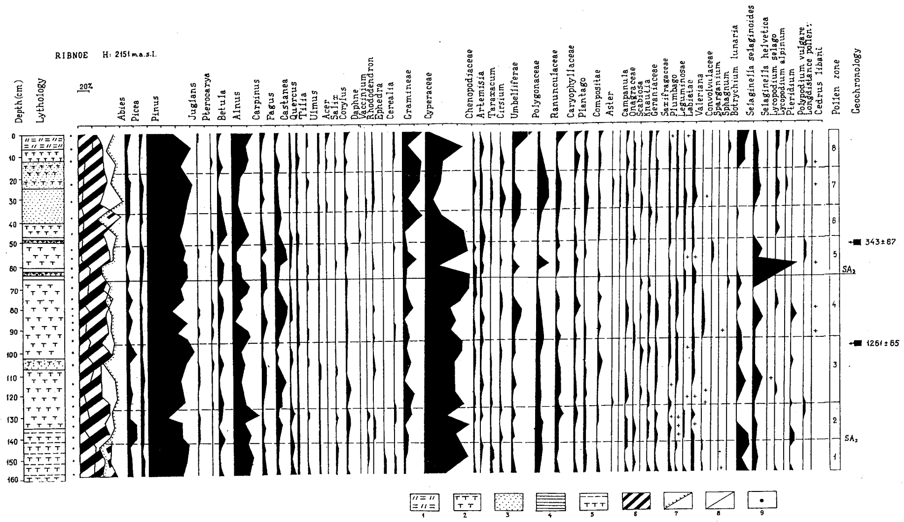
Fig. 5. Spore-pollen spectra of the Rybnoe profile. 1-soil, 2-peat, 3-sand, 4-lake clays, 5-clay with peat, 6-AP, 7-NAP, 8-spores, 9-sampling site (6, 7, 8, 9 valid also for Figs 7 and 9)
