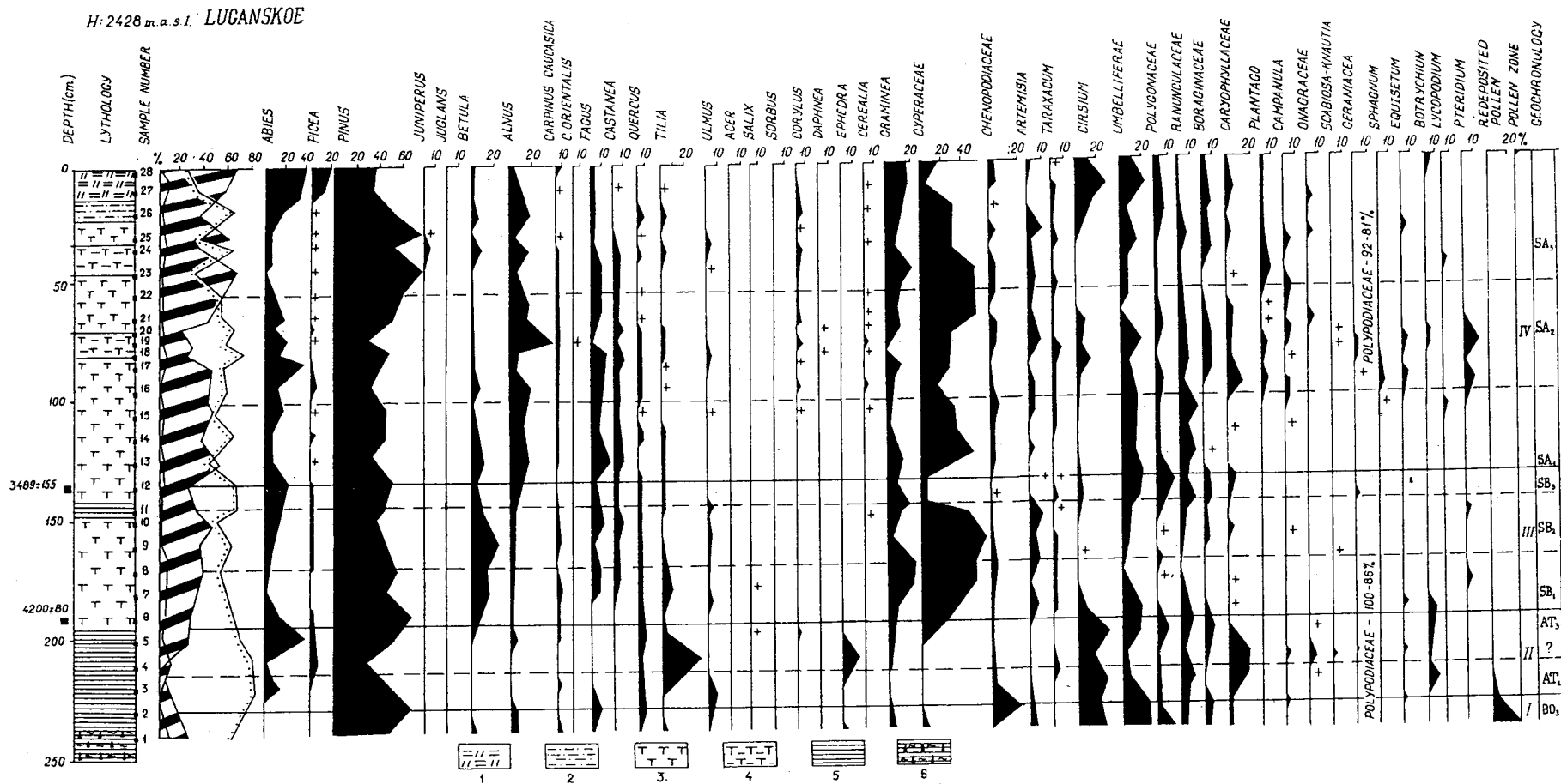
Fig. 7. Spore-pollen spectra of the Luganskoe profile. 1-soil, 2-clay with sand, 3-peat, 4-clay with peat, 5-lake clays, 6-clay with moraine
