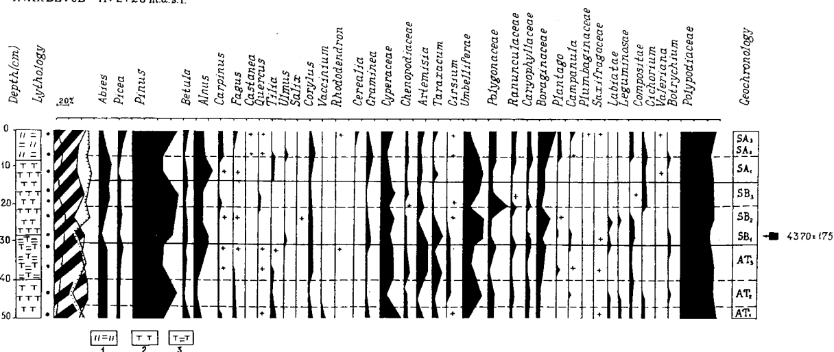
Fig. 8. Spore-pollen spectra of the Kvarzev0e profile. 1-soil, 2-peat, 3-clay with peat
