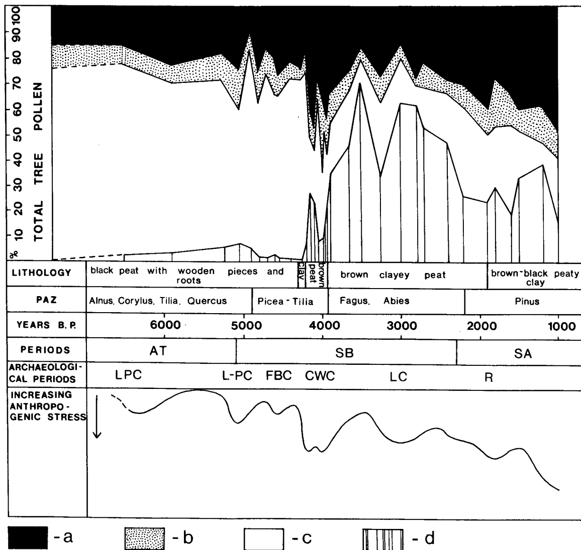
Fig. 9. Survey of the increasing anthropogenic stress. Cumulative tree pollen diagram, calculation sum recalculated (Andersen 1970, 1973) a - fen wood \Sigma Alnus : 4, Salix ; b - early successional \Sigma Corylus : 4, Betula : 4, Sambucus ; c - late successional \Sigma Ulmus : 2, Tilia \times 2, Quercus : 4, Fraxinus \times 2, Acer \times 2; d - \Sigma Fagus , Carpinus : 3, Abies ; LPC - Linear Pottery Culture, L-PC - Langyel - Polgar Cycle, FBC - Funnel Beaker Culture, CWC - Corded Ware Culture, LC - Lusatian Culture, R - Roman Period
