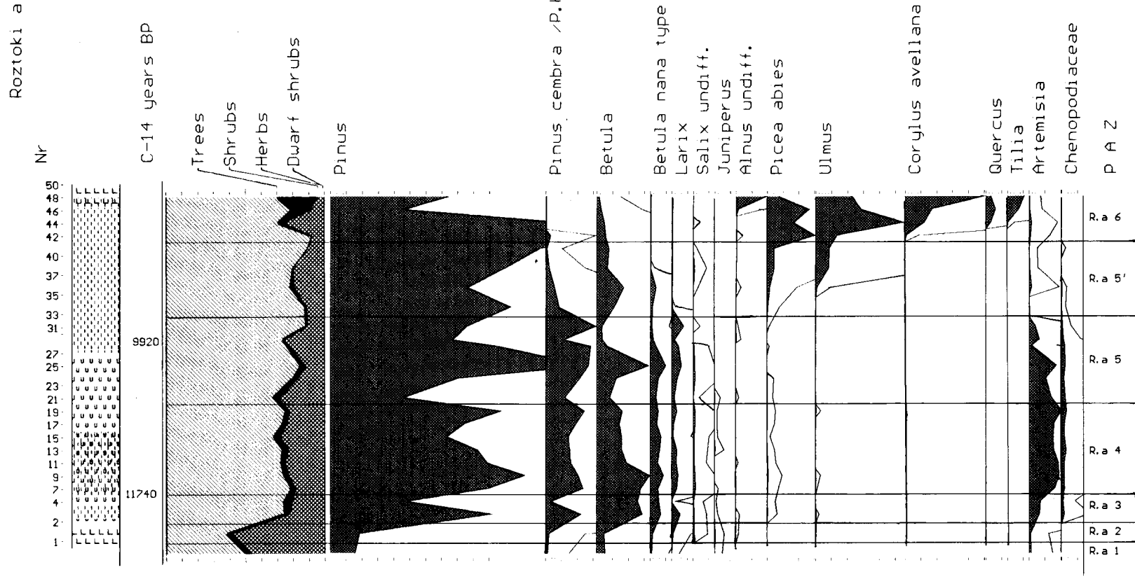
Fig. 4. Pollen concentration diagram from Roztoki a. Lithology see Fig. 3
