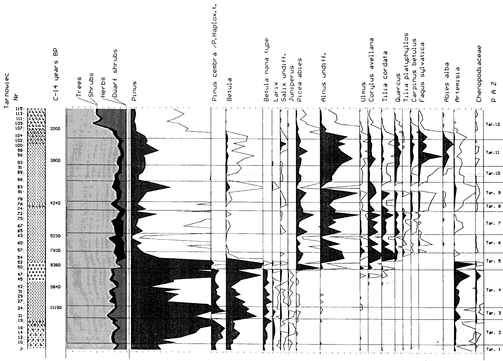
Fig. 6. Pollen concentration diagram from Tarnowiec. Lithology see Fig. 3
