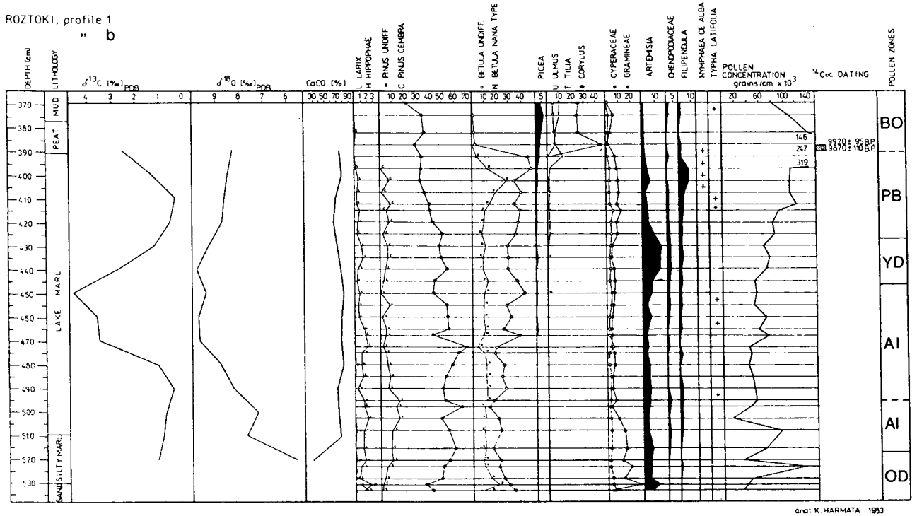
Fig. 8. Isotope and pollen diagram from Roztoki b fossil lake
