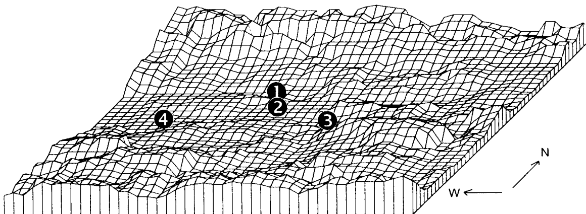
Fig. 2. The morphology of the investigation area (side of square - 13 km; altitude: 220-370 m a.s.l.) 1 - Roztoki a, 2 - Roztoki b, 3 - Tarnowiec, 4 - Jasło
