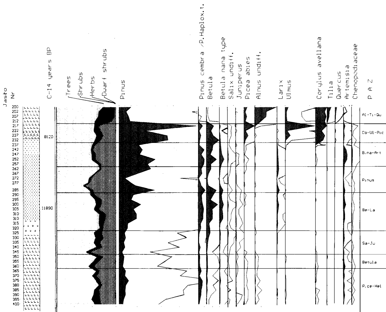
Fig. 7. Pollen concentration diagram from Jasło. Lithology see Fig. 3
