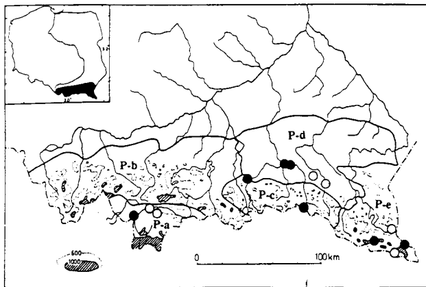
Fig. 1. The subdivision of the Polish Carpathians into palaeoecological type region (Ralska-Jasiewiczowa 1986). P-a – Tatra Mts., P-b – Western Beskidy Mts., P-c – Low Beskidy Mts., P-d – Jasło-Sanok Depression and eastern forelands, P-e – Bieszczady Mts. (● IGCP 158 reference sites, ○ additional sites)
