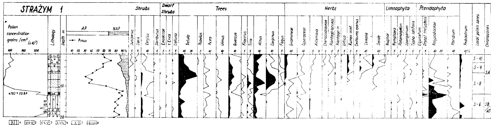
Fig. 4. Simplified pollen diagram from the Lake Strażym profile 1, selected pollen taxa. 1 — peat with clay, 2 — calcareous gyttja, 3 — clayey gyttja, 4 — clayey calcareous gyttja, 5 — sand with organic matter, 6 — sand
