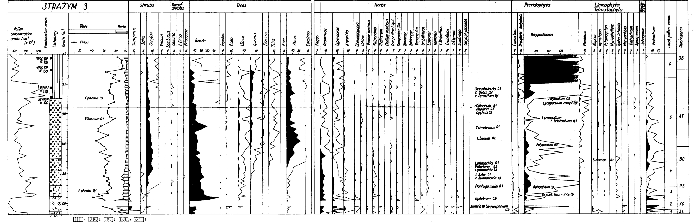
Fig. 3. Pollen diagram from the Lake Strażym profile 3. 1 — peat, 2 — calcareous gyttja, 3 — silty — calcareous gyttja, 4 — clayey — calcareous gyttja, 5 — sand
