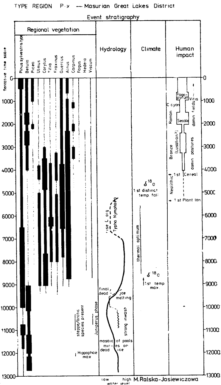
Fig. 2. The event stratigraphy table for the Masurian Great Lakes District type region
