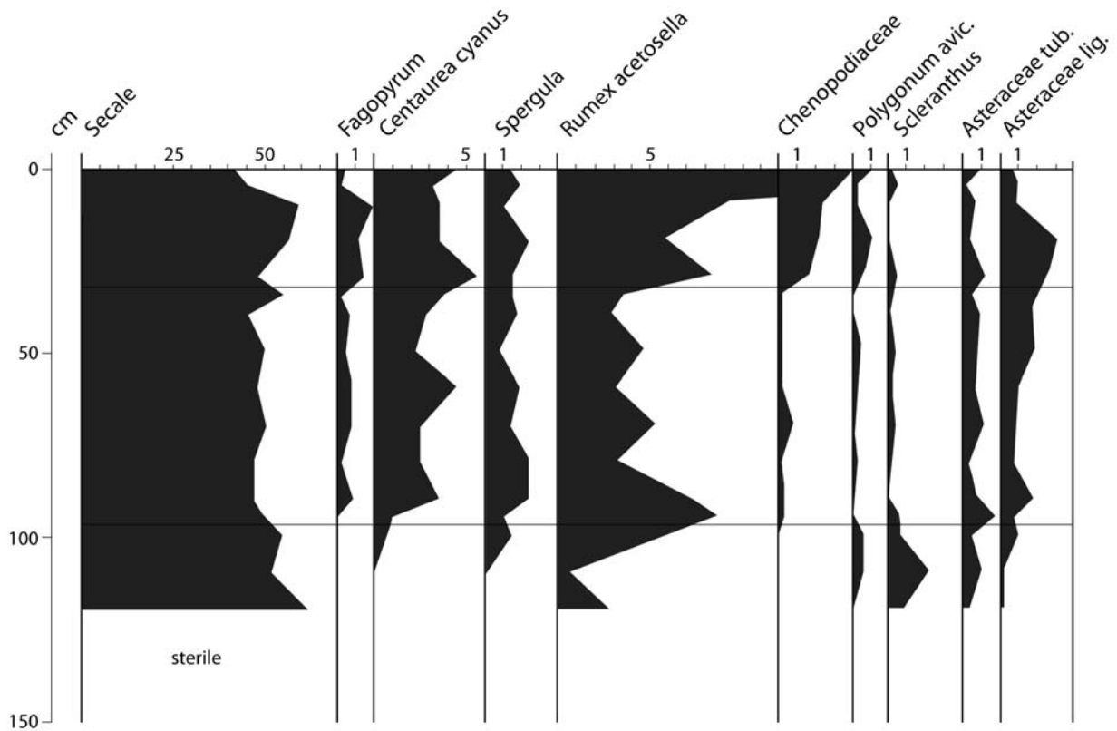
Fig. 4. Pollen diagram of the plaggen soil at Son en Breugel (Netherlands), selection of curves
